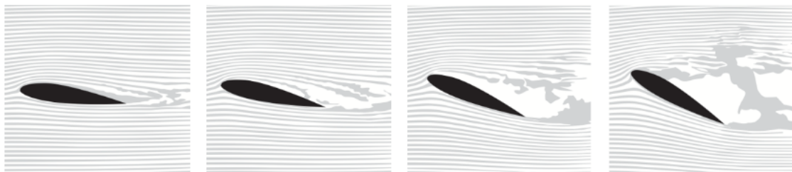
Figure 3. The wing stalls at critical angle of attack. This angle is always the same (for a given flap setting), whereas stall speed varies with gross weight and g load.
