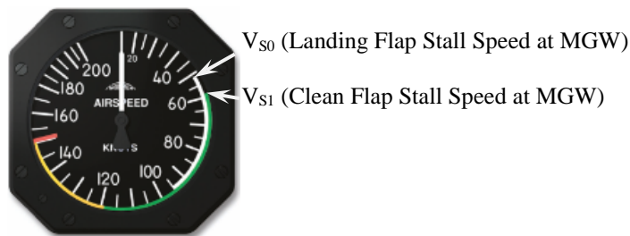
Figure 1. Conventional airspeed indicator LSA markings
